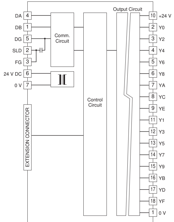
Output Circuit
