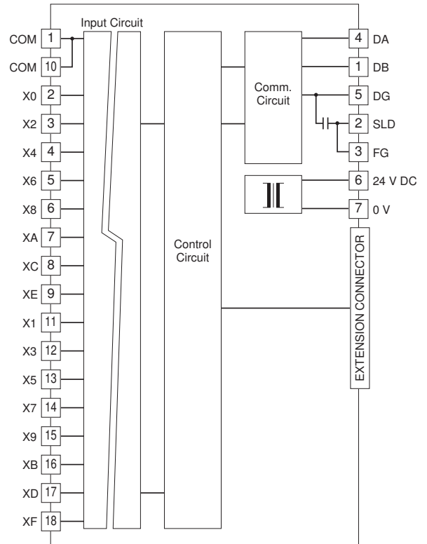
Input Circuit
