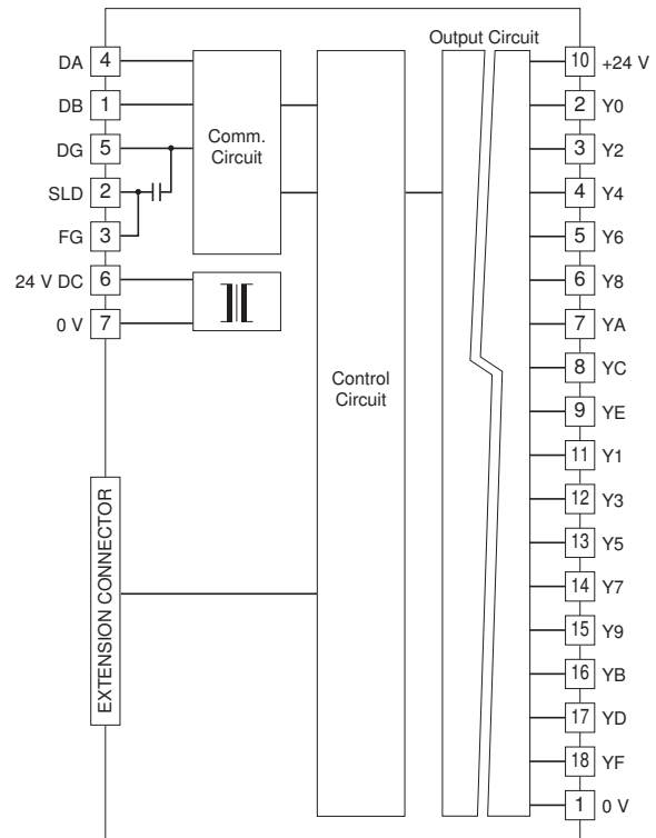
Output Circuit
