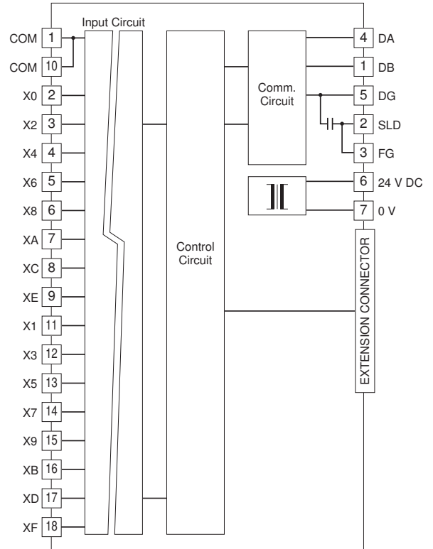
Input Circuit
