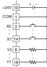
■ I/O Connection Example
