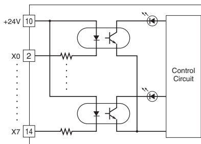
■ Output Circuit
