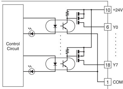
■ I/O Connection Example
