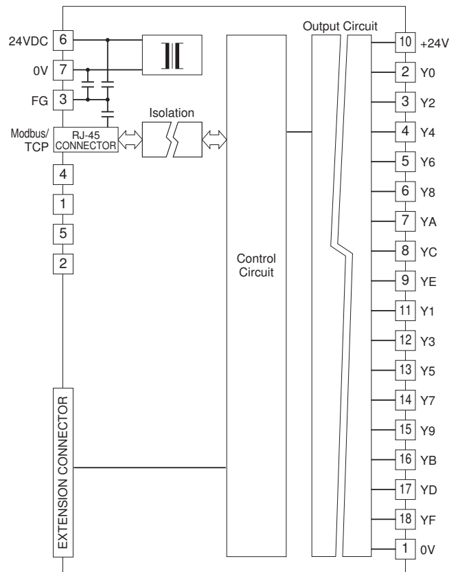
Output Circuit
