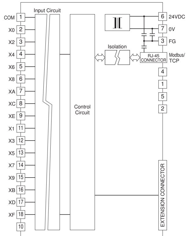
Input Circuit
