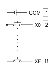
NPN Connection
