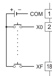
PNP Connection
