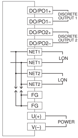
Discrete Output Connection E.g.
