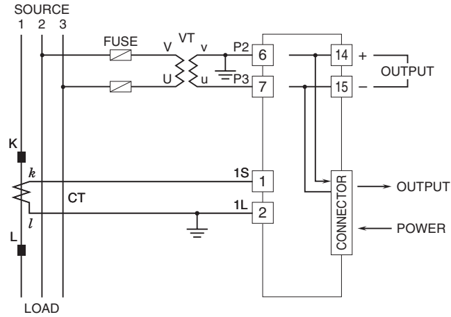
■ 3-PHASE/3-WIRE
